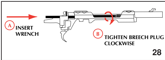
REPLACING THE BREECH PLUG
