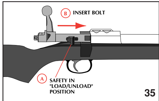
REINSERT BOLT
