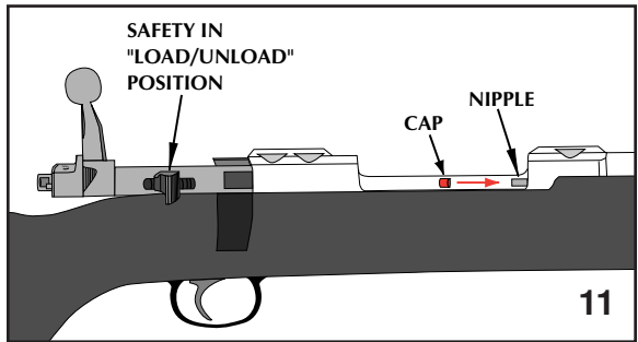
CAPPING THE NIPPLE
